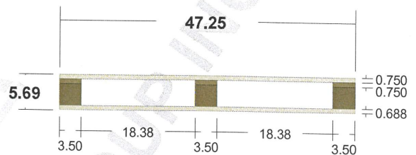
End View
